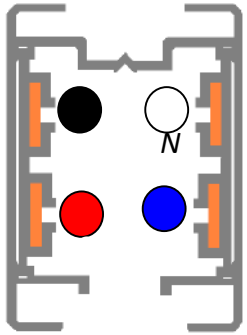
Four Pole
