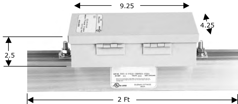
D. for Top Center Feed - CFB Series
