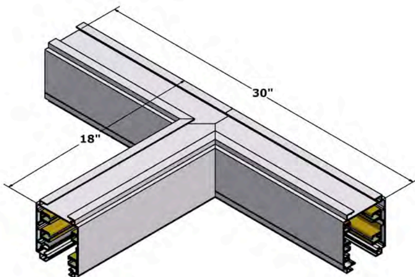
Internal Right -IR
