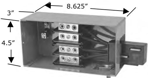
With Built-In Connector - EPF Series
