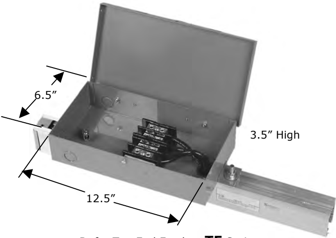
B. for Top End Feed - TF Series
